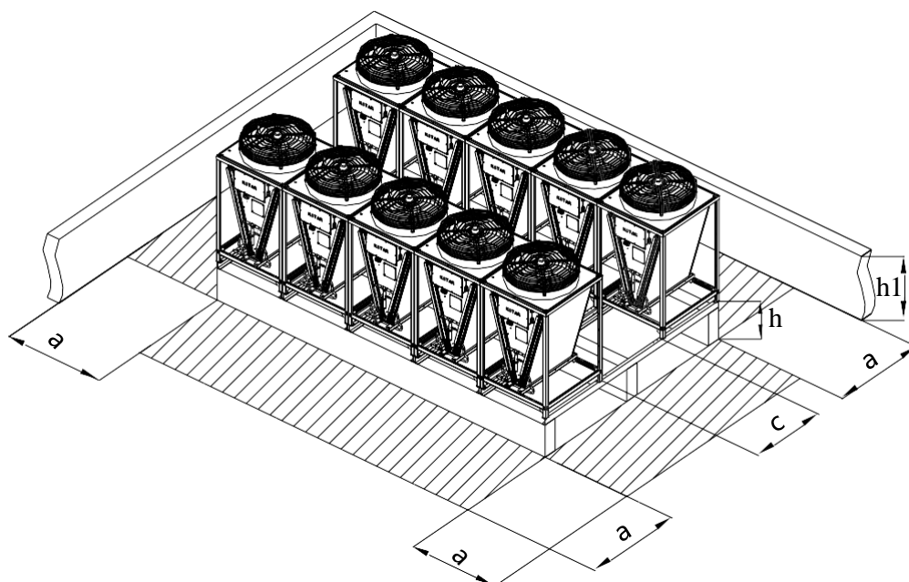
Fig. 2-3 EACCOND032*~096* Schematic diagram of V-Type installation
