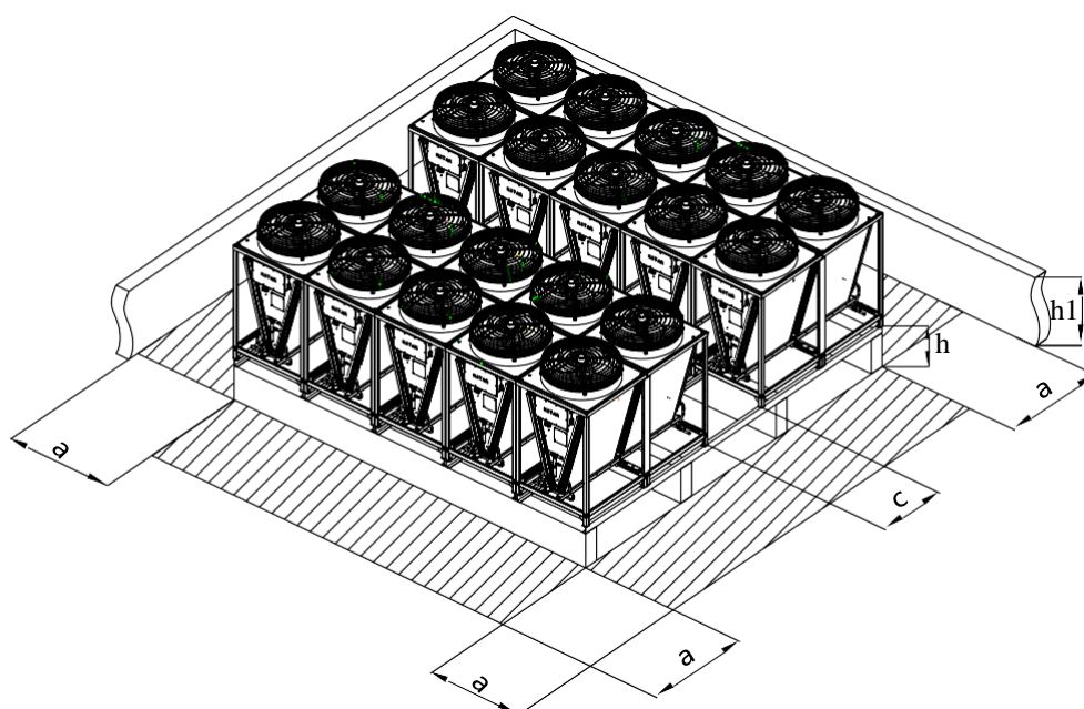
Fig.2-4 EACCOND108*~170* Schematic diagram of V-Type installation
