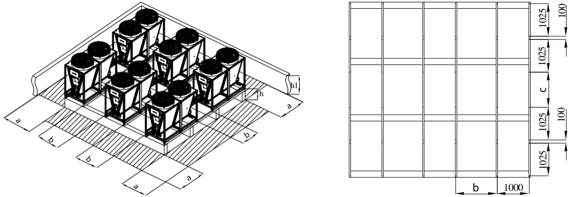
Fig.2-7 EACCOND108*~170* Spread-out distribution base bracket dimensions
