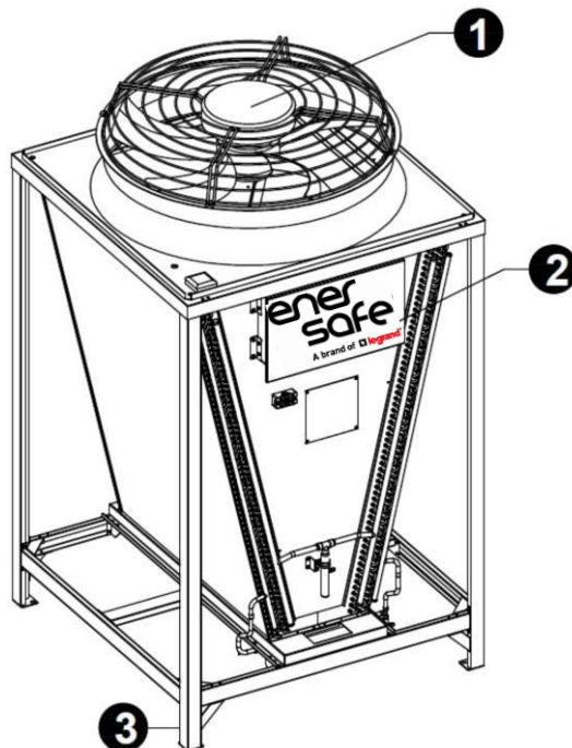
Fig. 1-2 Schematic diagram of single system of ECOND air-cooled V-Type condenser (single fan)
