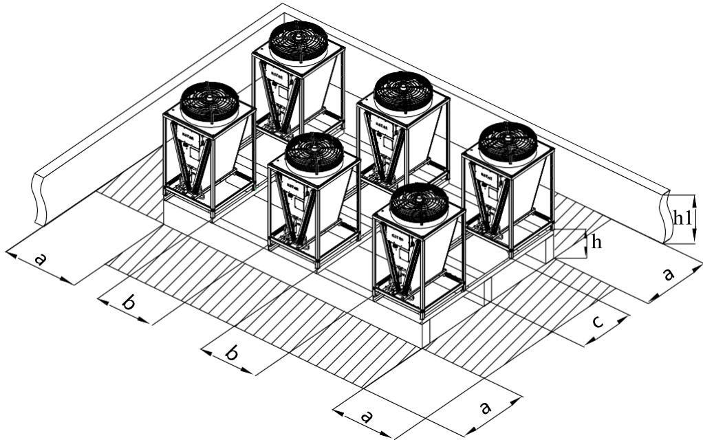
Fig. 2-1 EACCOND032*~096* Schematic diagram of dispersion distribution
