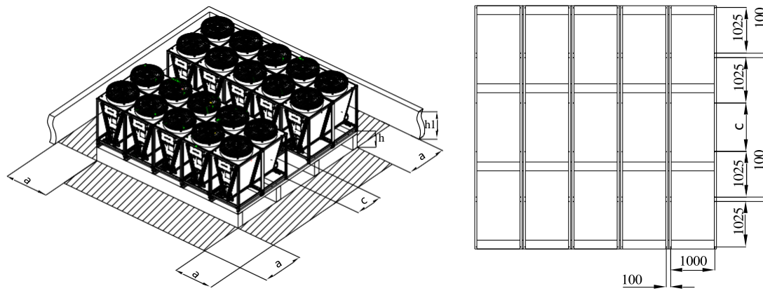
Fig.2-9 EACCOND108*~170* Side-by-side mounting base bracket dimensions
