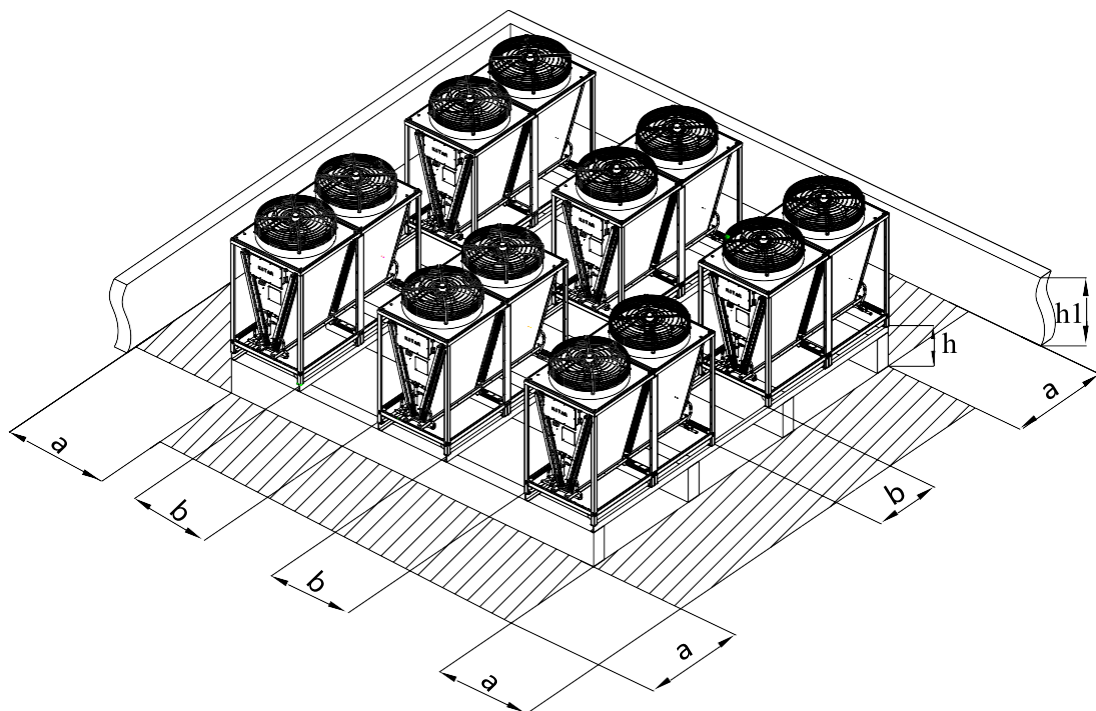
Fig. 2-2 EACCOND108*~170* Schematic diagram of dispersion distribution
