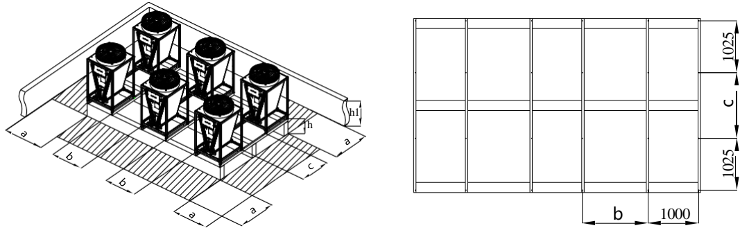
Fig.2-6 EACCOND032*~096* Spread-out distribution base bracket dimensions
