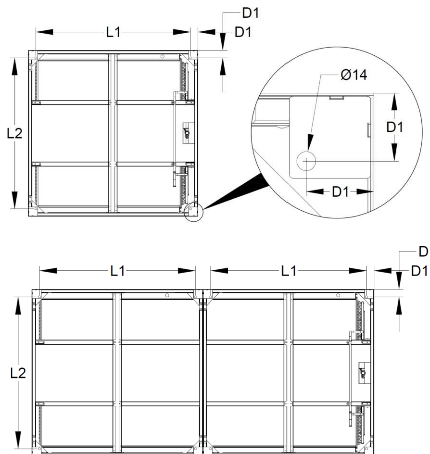
Fig. 1-5 Dimensions of the V-Type machine vertical support foot vacancy
