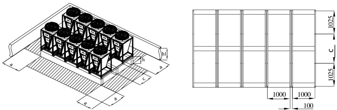
Fig.2-8 EACCOND032*~096* Side-by-side mounting base bracket dimensions
