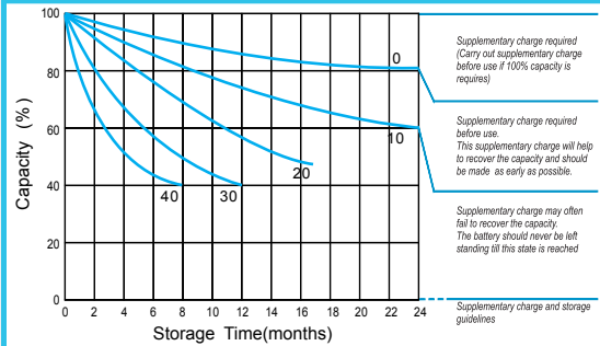
Storage Characteristics
